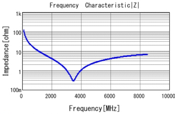
■ GRM0225C1H130GA03 |Z| DCOV, 25degC
