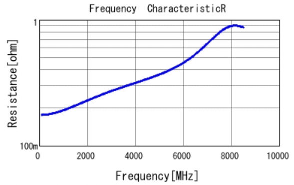
■ GRM0225C1H130GA03 R DCOV, 25degC
