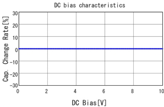
■ GRM1557U1A332JA01 C-DC bias capchange, 25.0degC, AC1V
