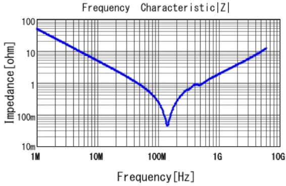
■ GRM1557U1A332JA01 |Z| DCOV, 25degC
