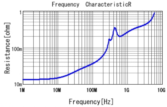
■ GRM1557U1A332JA01 R DCOV, 25degC
