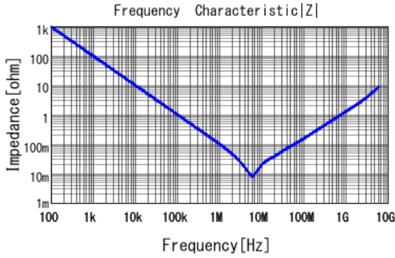
■ GRM155C80J225KE95 |Z| DCOV, 25degC
