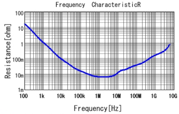
■ GRM155C80J225KE95 R DCOV, 25degC
