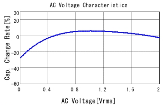
■ GRM155C80J225KE95 C-AC Voltage capchange, DCOV, 25.0d
