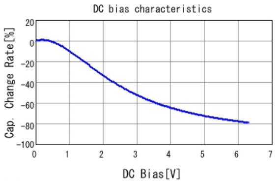
■ GRM155C80J225KE95 C-DC bias capchange, 25.0degC, AC0.
