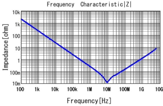
■ GRM155C71A105KE11 |Z| DCOV, 25degC
