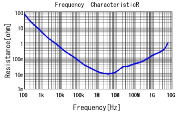
■ GRM155C71A105KE11 R DCOV, 25degC
