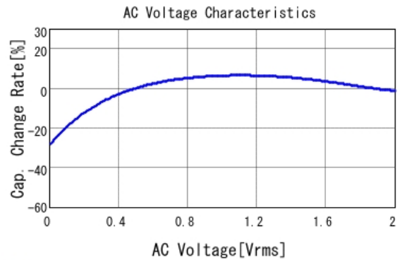
■ GRM153R61A105ME95 C-AC Voltage capchange, DCOV, 25.0d
