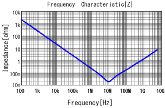
■ GRM153R61A105ME95 |Z| DCOV, 25degC
