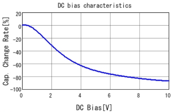
■ GRM153R61A105ME95 C-DC bias capchange, 25.0degC, AC0.
