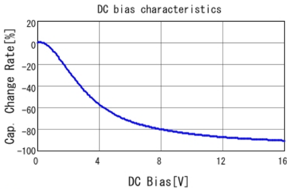
■ GRM155R61C225KE44 C-DC bias capchange, 25.0degC, AC1V
