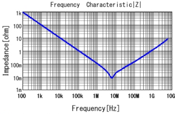
■ GRM155R61C225KE44 |Z| DCOV, 25degC
