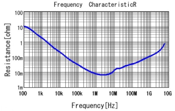
■ GRM155R61C225KE44 R DCOV, 25degC
