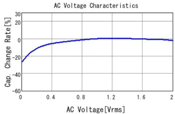
■ GRM155R61C225KE44 C-AC Voltage capchange, DCOV, 25.0d
