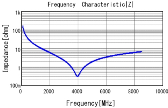
■ GRM0225C1H100GA03 |Z| DCOV, 25degC
