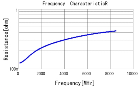
■ GRM0225C1H100GA03 R DCOV, 25degC
