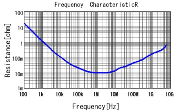
■ GRM153R60J225ME95 R DCOV, 25degC
