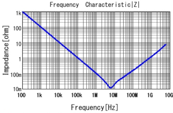
■ GRM153R60J225ME95 |Z| DCOV, 25degC
