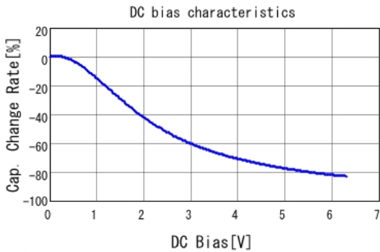
■ GRM153R60J225ME95 C-DC bias capchange, 25.0degC, ACO.
