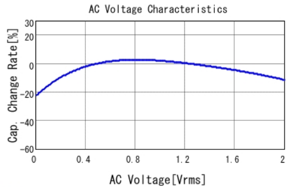
■ GRM153R60J225ME95 C-AC Voltage capchange, DCOV, 25.0d
