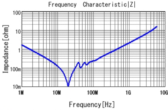
■ GRM21B7U1A104JA01 |Z| DCOV, 25degC
