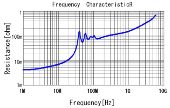
■ GRM21B7U1A104JA01 R DCOV, 25degC
