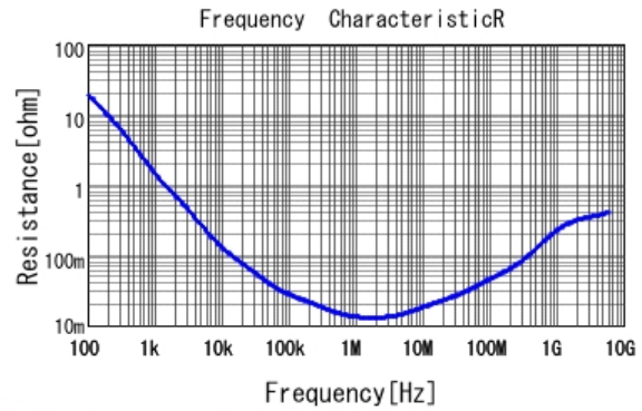
■ GRM155D80J225KE95 R DC0V, 25degC
