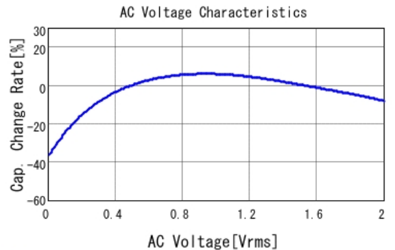
■ GRM155D80J225KE95 C-AC Voltage capchange, DC0V, 25.0d
