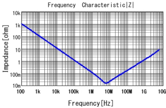
■ GRM155D80J225KE95 |Z| DC0V, 25degC
