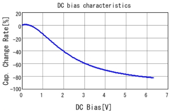
■ GRM155D80J225KE95 C-DC bias capchange, 25.0degC, AC0.
