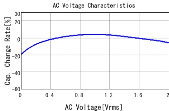
■ GRM155R60J225KE01 C-AC Voltage capchange, DCOV, 25.0d
