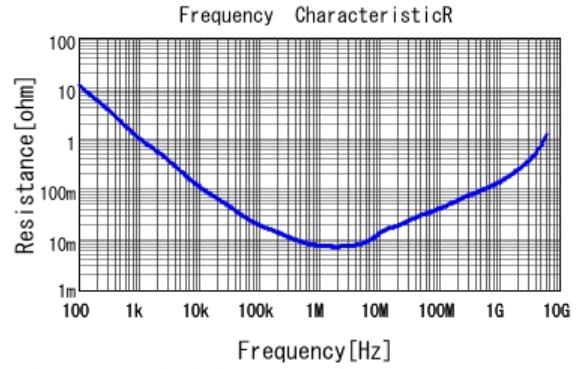
■ GRM155R60J225KE01 R DCOV, 25degC
