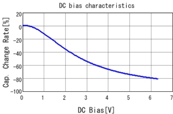
■ GRM155R60J225KE01 C-DC bias capchange, 25.0degC, AC0.
