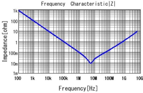
■ GRM155R60J225KE01 |Z| DCOV, 25degC
