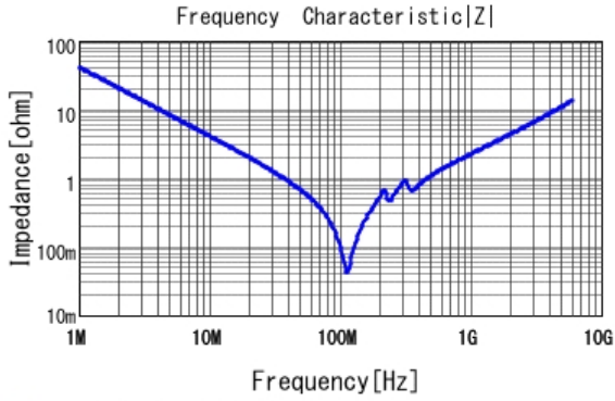
■ GRM1885C1H392JA01 |Z| DCOV, 25degC
