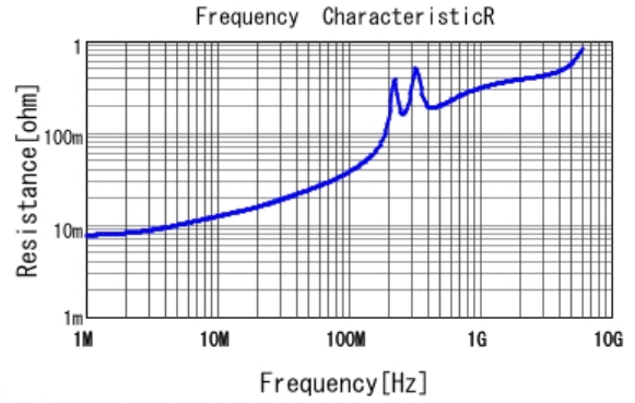
■ GRM1885C1H392JA01 R DCOV, 25degC
