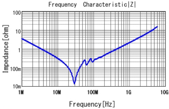
■ GRM21B7U1H473JA01 |Z| DCOV, 25degC
