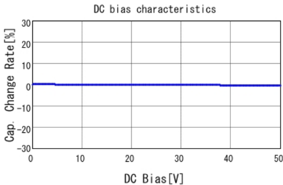
■ GRM21B7U1H473JA01 C-DC bias capchange, 25.0degC, AC1V
