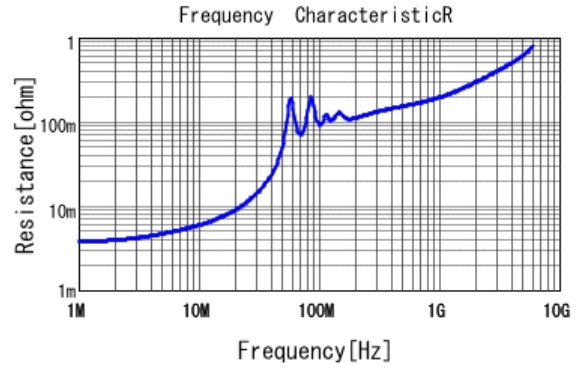
■ GRM21B7U1H473JA01 R DCOV, 25degC
