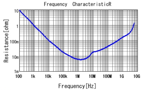
■ GRM185C80J475ME11 R DCOV, 25degC
