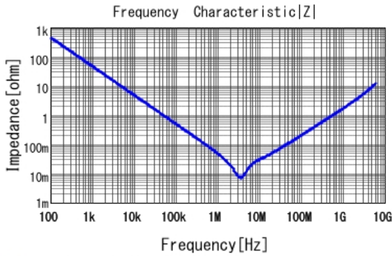
■ GRM185C80J475ME11 |Z| DCOV, 25degC
