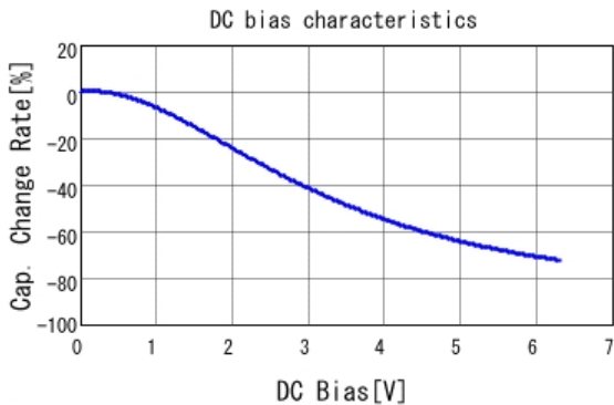
■ GRM185C80J475ME11 C-DC bias capchange, 25.0degC, ACO.
