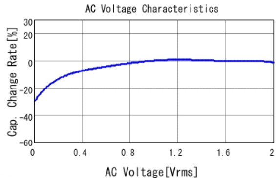
■ GRM185C80J475ME11 C-AC Voltage capchange, DCOV, 25.0d
