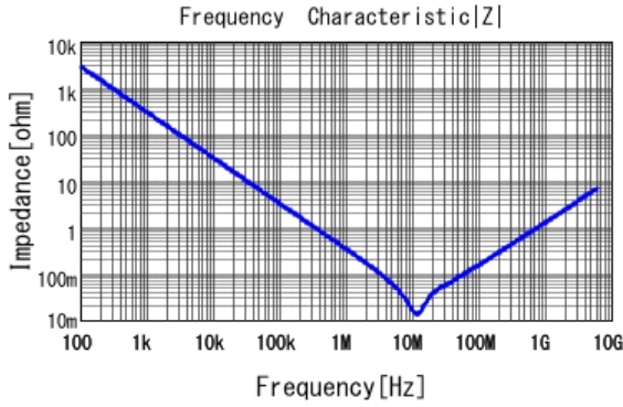
■ GRM155C81C105KE15 |Z| DCOV, 25degC
