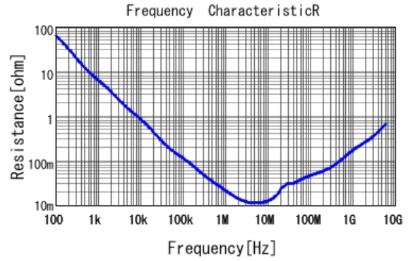
■ GRM155C81C105KE15 R DCOV, 25degC
