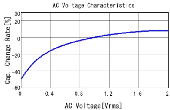
■ GRM155C81C105KE15 C-AC Voltage capchange, DCOV, 25.0d
