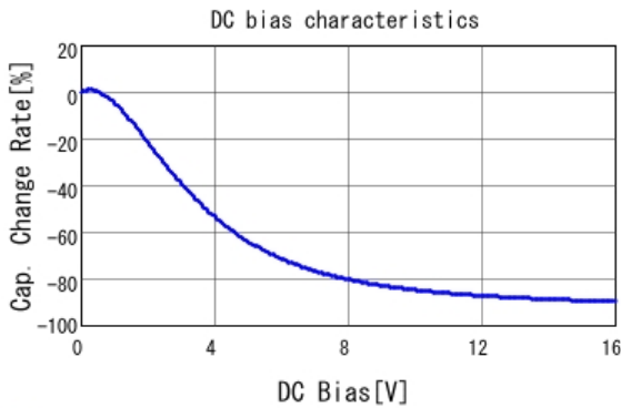
■ GRM155C81C105KE15 C-DC bias capchange, 25.0degC, AC1.
