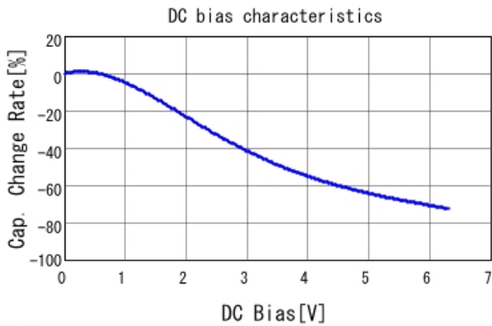
■ GRM155C80J475MEAA C-DC bias capchange, 25.0degC, ACO.
