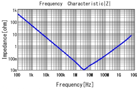
■ GRM155C80J475MEAA |Z| DCOV, 25degC
