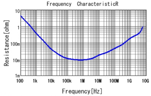
■ GRM155C80J475MEAA R DCOV, 25degC
