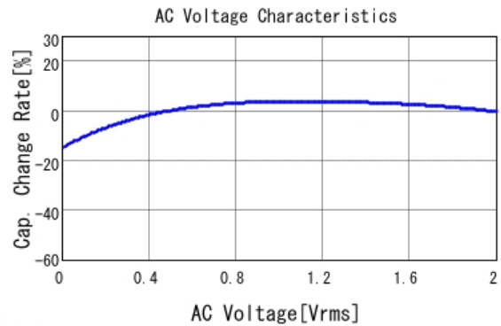
■ GRM155C80J475MEAA C-AC Voltage capchange, DCOV, 25.0d
