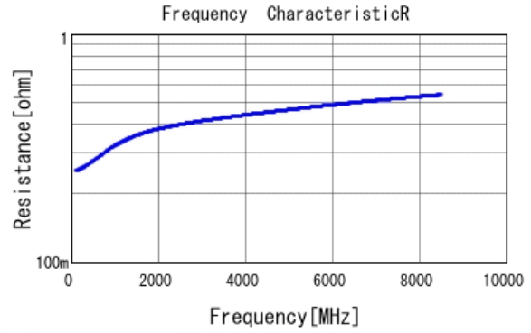
■ GRM0225C1H2R1CA03 R DCOV, 25degC
