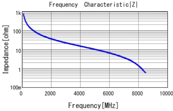
■ GRM0225C1H2R1CA03 |Z| DCOV, 25degC
