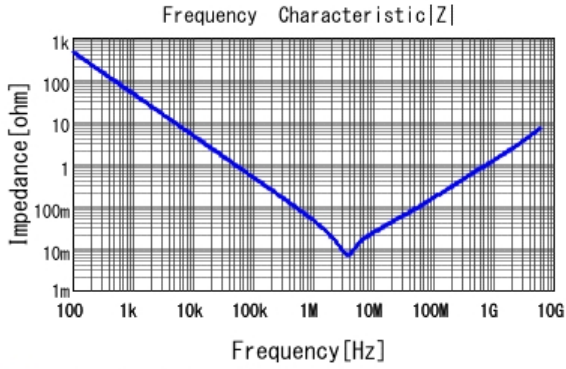
■ GRM155D80E475ME47 |Z| DCOV, 25degC
