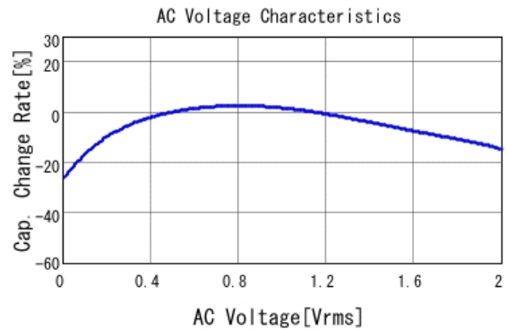
■ GRM155D80E475ME47 C-AC Voltage capchange, DCOV, 25.0d
