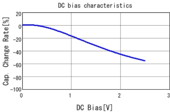
■ GRM155D80E475ME47 C-DC bias capchange, 25.0degC, AC0.
