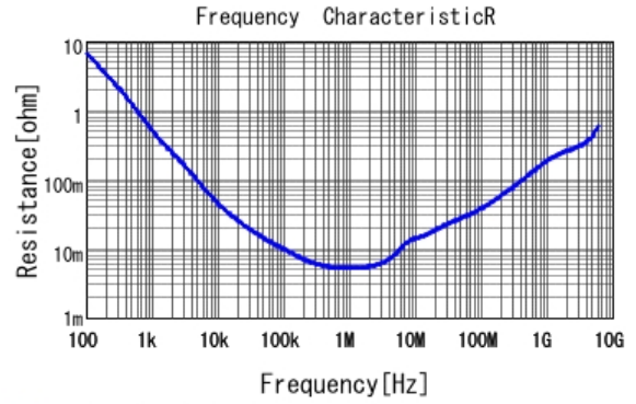
■ GRM155D80E475ME47 R DCOV, 25degC
