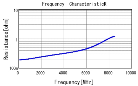
■ GRM0225C1H120GA03 R DCOV, 25degC
