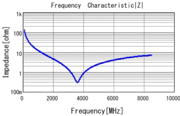
■ GRM0225C1H120GA03 |Z| DCOV, 25degC
