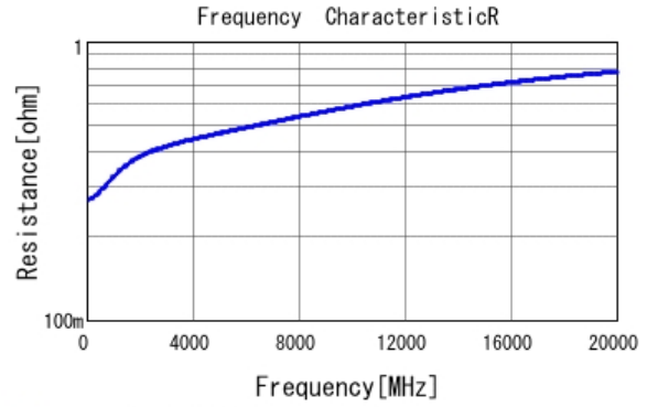
■ GRM0225C1H2R0BA03 R DCOV, 25degC
