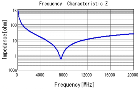
■ GRM0225C1H2R0BA03 |Z| DCOV, 25degC
