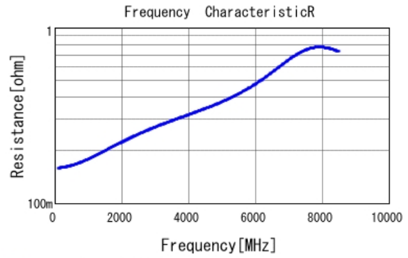
■ GRM0225C1H150GA03 R DCOV, 25degC
