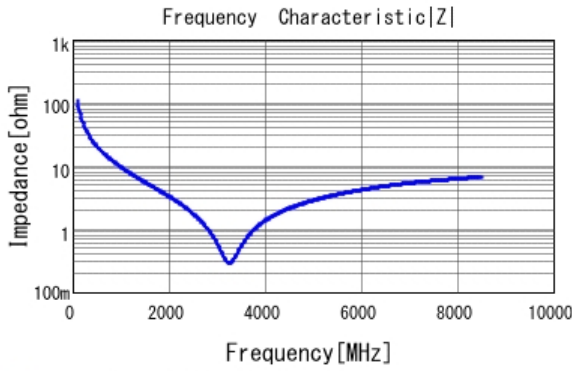
■ GRM0225C1H150GA03 |Z| DCOV, 25degC
