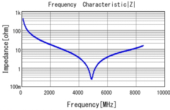
■ GJM0335C1E3R9BB01 |Z| DC0V, 25degC
