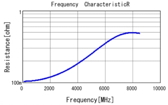
■ GJM0335C1E3R9BB01 R DC0V, 25degC
