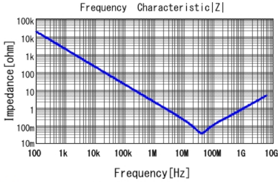
■ GRM022R61A104ME01 |Z| DCOV, 25degC
