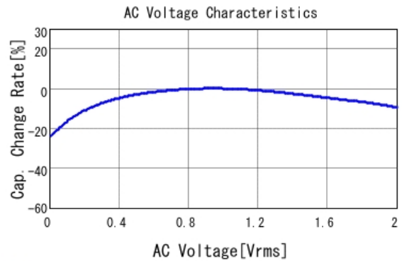
■ GRM022R61A104ME01 C-AC Voltage capchange, DCOV, 25.0d
