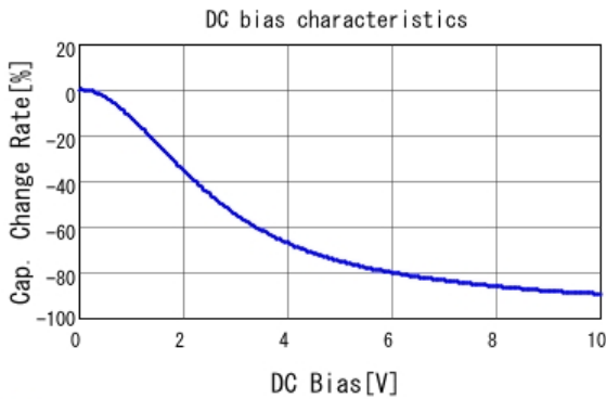
■ GRM022R61A104ME01 C-DC bias capchange, 25.0degC, AC1V
