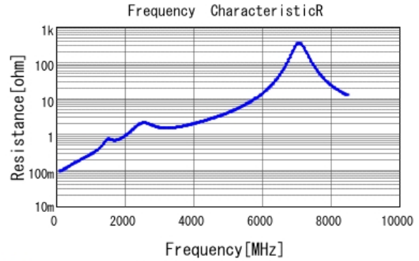
■ GCM1885C2A121JA16 R DCOV, 25degC
