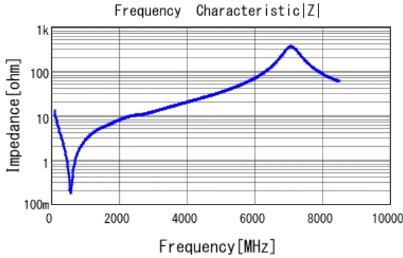
■ GCM1885C2A121JA16 |Z| DCOV, 25degC
