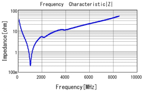
■ GCM1885C2A470JA16 |Z| DCOV, 25degC
