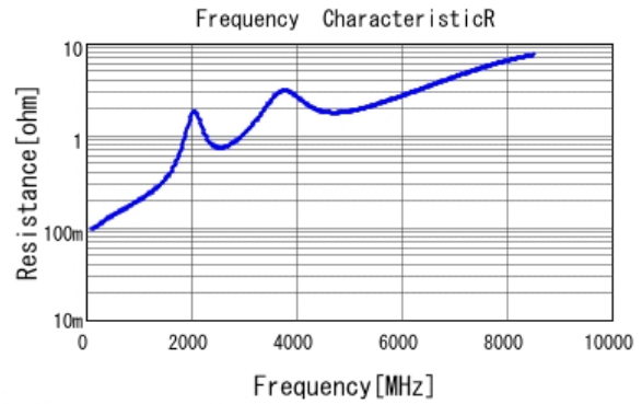
■ GCM1885C2A470JA16 R DCOV, 25degC
