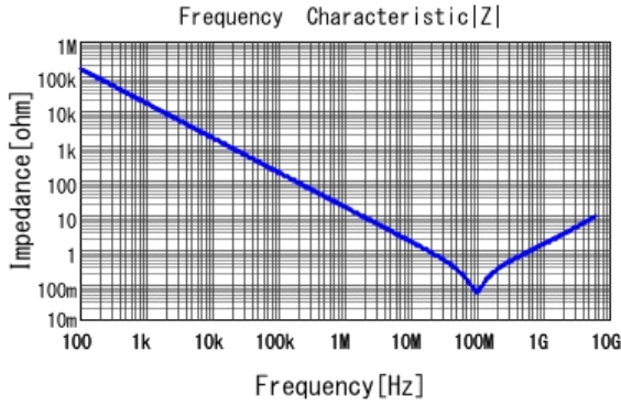
■ GRM033R61E103KA12 |Z| DCOV, 25degC
