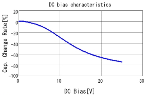
■ GRM033R61E103KA12 C-DC bias capchange, 25.0degC, AC1.
