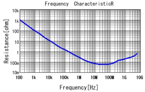
■ GRM033R61E103KA12 R DCOV, 25degC
