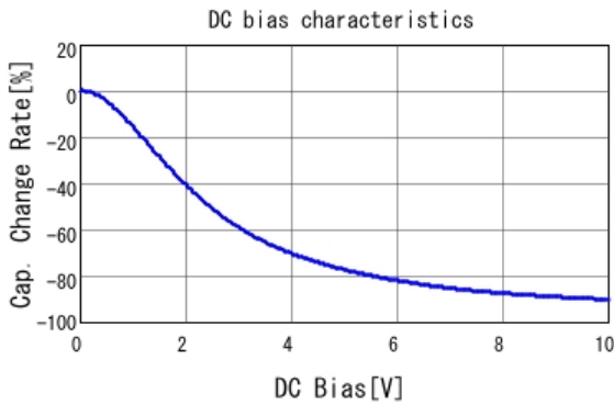
■ GRM033R61A225ME47 C-DC bias capchange, 25.0degC, AC1V
