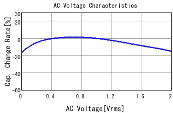
■ GRM033R61A225ME47 C-AC Voltage capchange, DCOV, 25.0d
