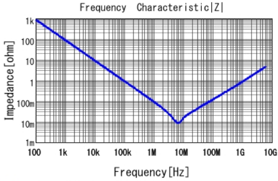
■ GRM033R61A225ME47 |Z| DCOV, 25degC
