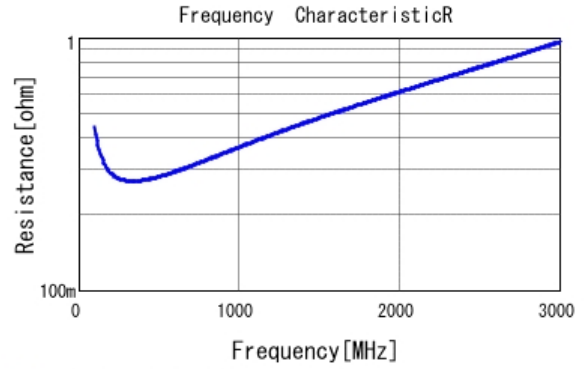
■ GCM21A5C2E100JX01 R DC0V, 25degC
