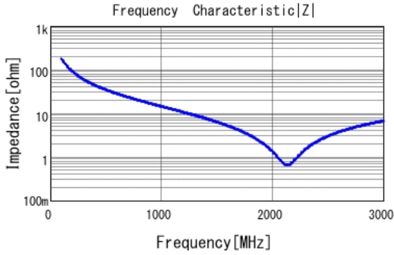
■ GCM21A5C2E100JX01 |Z| DC0V, 25degC
