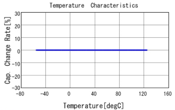
■ GCM21A5C2E471JX01 C-Temp. capchange, DC0V, AC1Vrms
