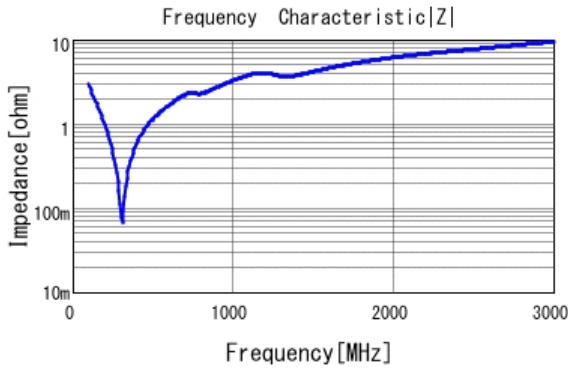
■ GCM21A5C2E471JX01 |Z| DC0V, 25degC
