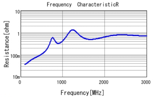
■ GCM21A5C2E471JX01 R DC0V, 25degC
