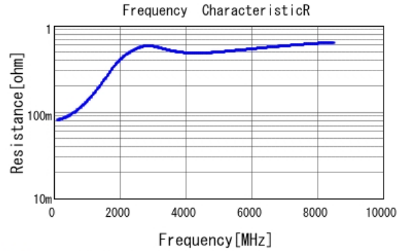
■ GRM0225C1E221JA02 R DCOV, 25degC
