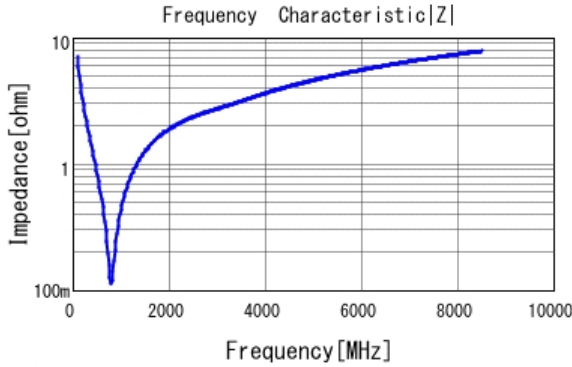
■ GRM0225C1E221JA02 |Z| DCOV, 25degC
