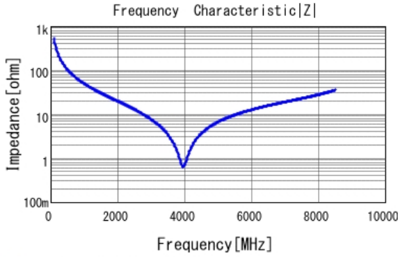
■ GCM1885C2A3R0CA16 |Z| DCOV, 25degC
