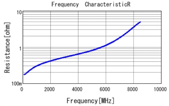
■ GCM1885C2A3R0CA16 R DCOV, 25degC
