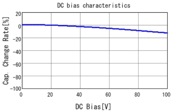
GCM2199E2A102KA05 C-DC bias capchange, 20.0degC, AC1V
