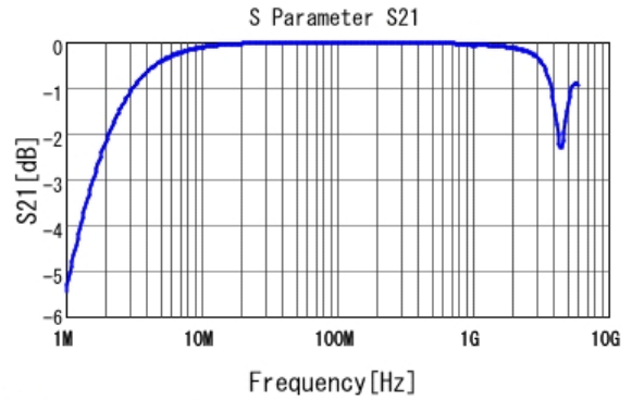
■ GCM2199E2A102KA05 S21 DC0V, 20degC
