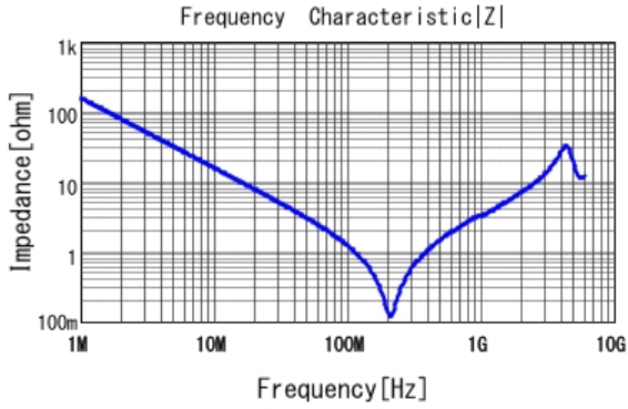
GCM2199E2A102KA05 |Z| DCOV, 20degC
