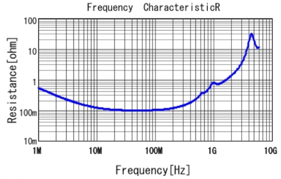
GCM2199E2A102KA05 R DCOV, 20degC
