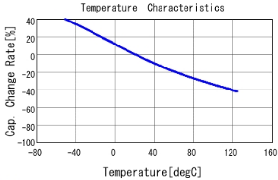
■ GCM2199E2A102KA05 C-Temp. capchange, DC0V, AC1Vrms
