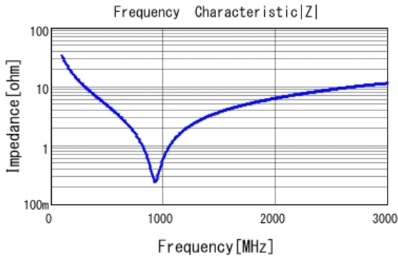
■ GCM21A5C2E470JX01 |Z| DC0V, 25degC
