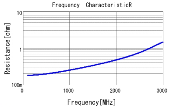
■ GCM21A5C2E470JX01 R DC0V, 25degC
