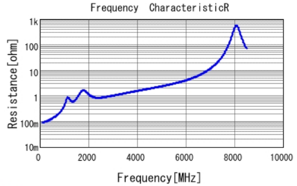
■ GCM1885C2A181JA16 R DCOV, 25degC
