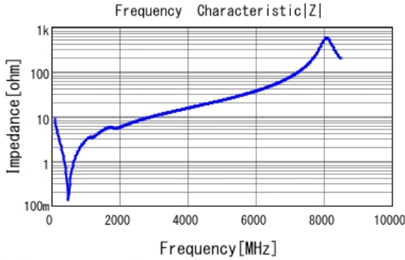
■ GCM1885C2A181JA16 |Z| DCOV, 25degC
