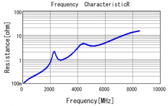
■ GCM1885C2A390JA16 R DCOV, 25degC
