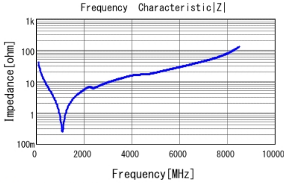
■ GCM1885C2A390JA16 |Z| DCOV, 25degC
