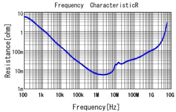
■ GRM188Z71C225KE43 R DCOV, 25degC
