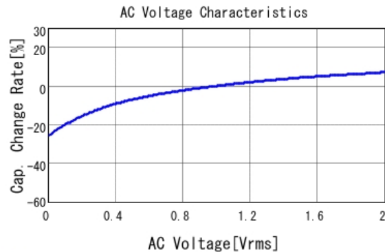
■ GRM188Z71C225KE43 C-AC Voltage capchange, DCOV, 25.0d
