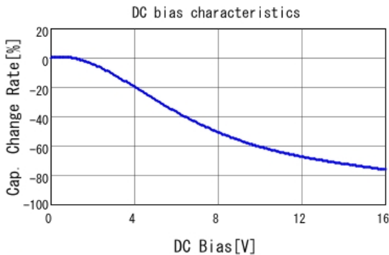
■ GRM188Z71C225KE43 C-DC bias capchange, 25.0degC, AC1V
