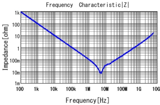
■ GRM188Z71C225KE43 |Z| DCOV, 25degC
