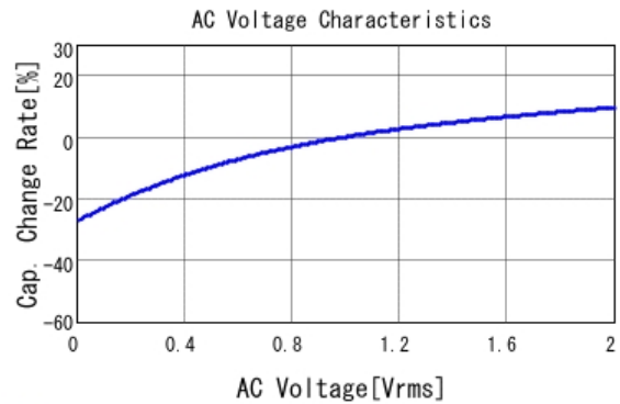
■ GRM21BC7YA475KE11 C-AC Voltage capchange, DCOV, 25.0d
