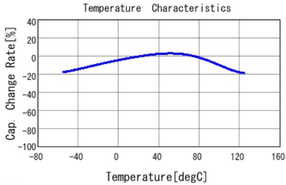
■ GRM21BC7YA475KE11 C-Temp. capchange, DC0.0V, AC0.5V rm
