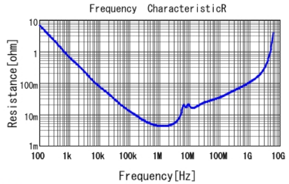
■ GRM21BC7YA475KE11 R DCOV, 25degC
