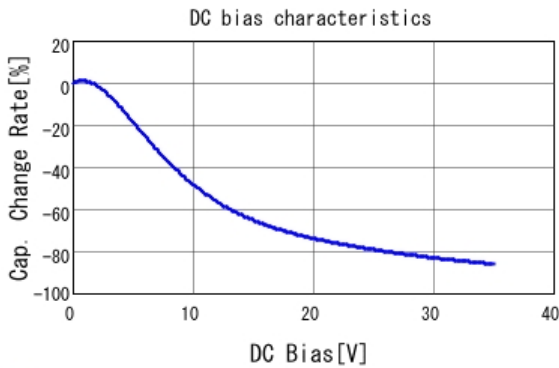
■ GRM21BC7YA475KE11 C-DC bias capchange, 25.0degC, AC1V
