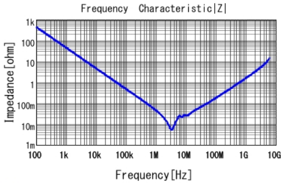
■ GRM21BC7YA475KE11 |Z| DCOV, 25degC
