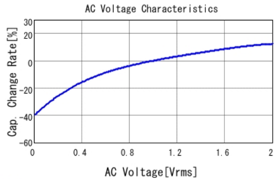
GCM188R71C105KA64 C-AC Voltage capchange, DCOV, 25.0d
