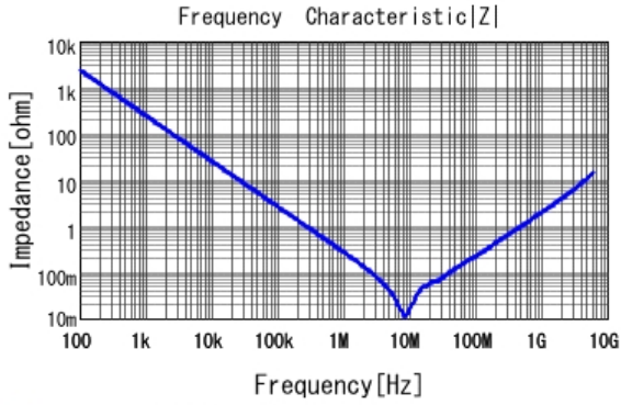
GCM188R71C105KA64 |Z| DCOV, 25degC
