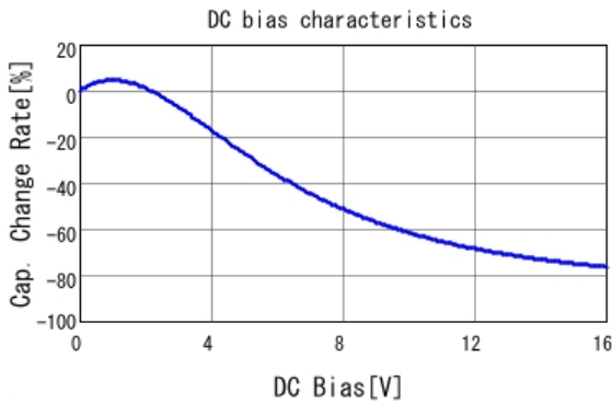
GCM188R71C105KA64 C-DC bias capchange, 25.0degC, AC1.
