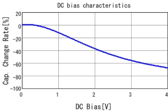
■ GRM188C80G226ME15 C-DC bias capchange, 25.0degC, AC0.
