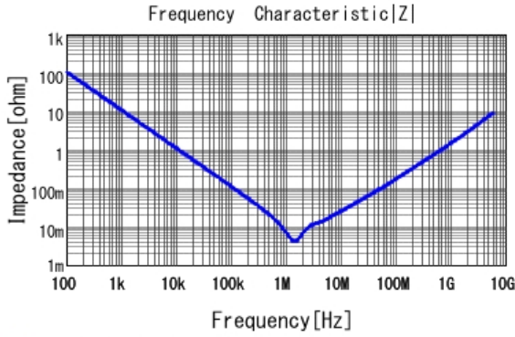
■ GRM188C80G226ME15 |Z| DCOV, 25degC
