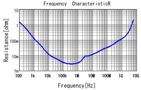
■ GRM188C80G226ME15 R DCOV, 25degC
