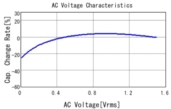
■ GRM188C80G226ME15 C-AC Voltage capchange, DCOV, 25.0d
