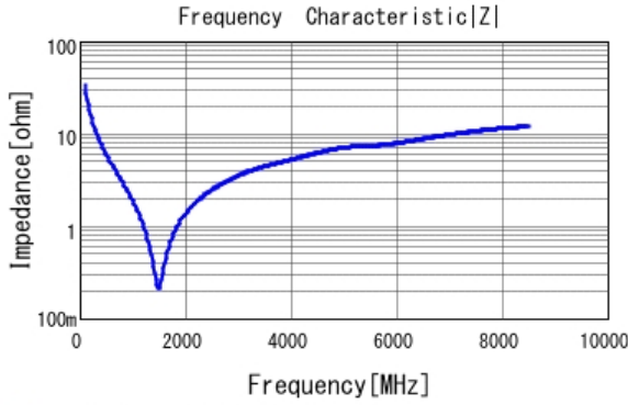
■ GRM0335C1H470GA01 |Z| DCOV, 25degC
