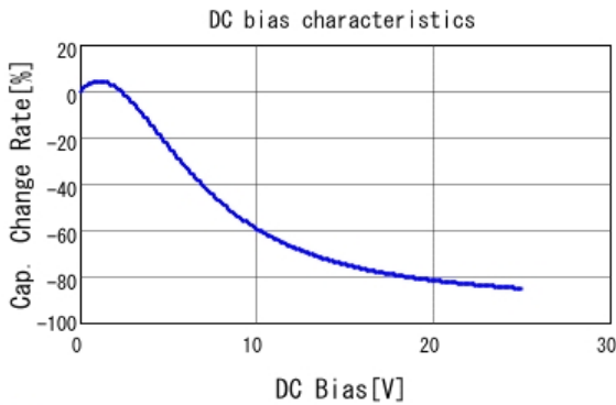
GCM188R71E105KA64 C-DC bias capchange, 25.0degC, AC1.
