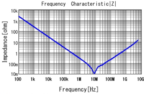
GCM188R71E105KA64 |Z| DC0V, 25degC
