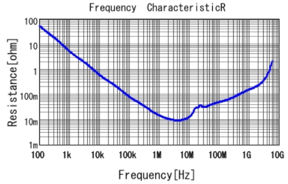
GCM188R71E105KA64 R DC0V, 25degC
