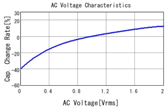
GCM188R71E105KA64 C-AC Voltage capchange, DC0V, 25.0d
