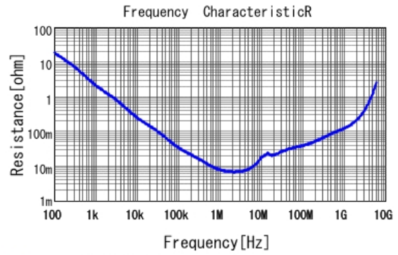
■ GRM188R61E225MA12 R DCOV, 25degC
