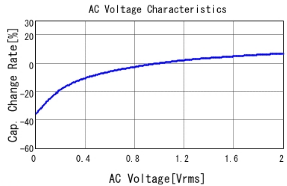
■ GRM188R61E225MA12 C-AC Voltage capchange, DCOV, 25.0d
