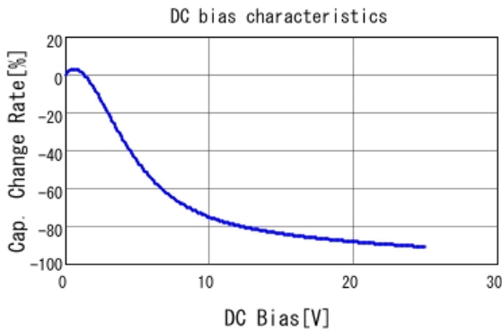
■ GRM188R61E225MA12 C-DC bias capchange, 25.0degC, AC1.
