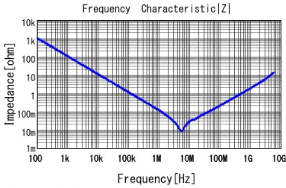
■ GRM188R61E225MA12 |Z| DCOV, 25degC
