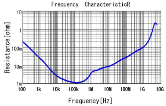
■ GRM21BC80G107ME15 R DCOV, 25degC
