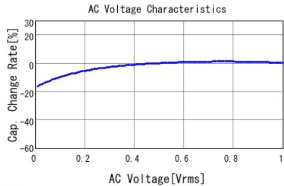
■ GRM21BC80G107ME15 C-AC Voltage capchange, DCOV, 25.0d
