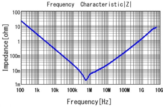
■ GRM21BC80G107ME15 |Z| DCOV, 25degC
