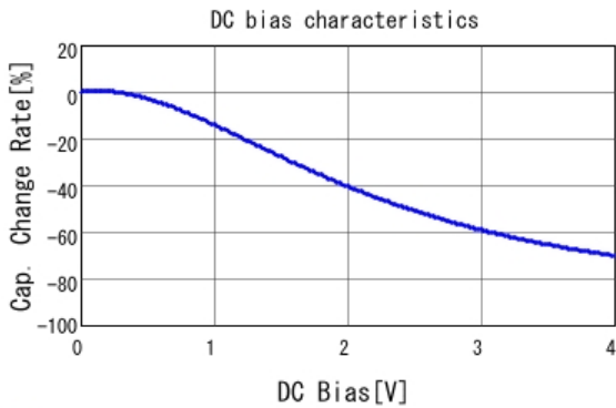
■ GRM21BC80G107ME15 C-DC bias capchange, 25.0degC, AC0.
