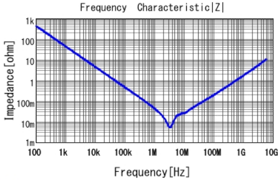
■ GRM188R6YA475ME15 |Z| DCOV, 25degC
