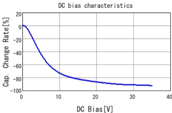
■ GRM188R6YA475ME15 C-DC bias capchange, 25.0degC, AC1V
