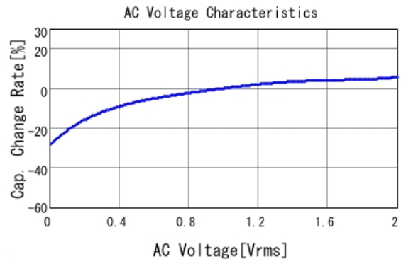
■ GRM188R6YA475ME15 C-AC Voltage capchange, DCOV, 25.0d
