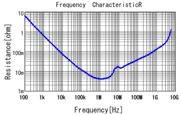
■ GRM188R6YA475ME15 R DCOV, 25degC
