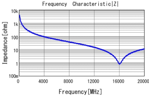
■ GRM0225C1HR40WA03 |Z| DCOV, 25degC
