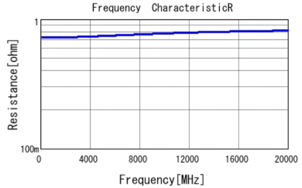
■ GRM0225C1HR40WA03 R DCOV, 25degC
