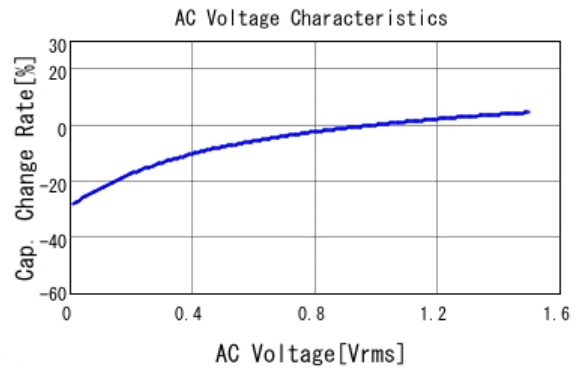
■ GRM21BC71C106KE11 C-AC Voltage capchange, DCOV, 25.0d
