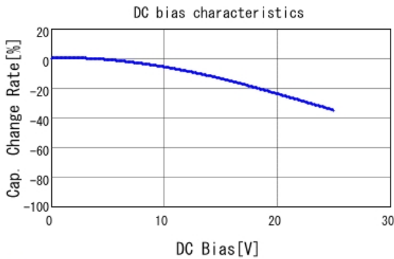
GCM188R71E154KA37 C-DC bias capchange, 25.0degC, AC1.
