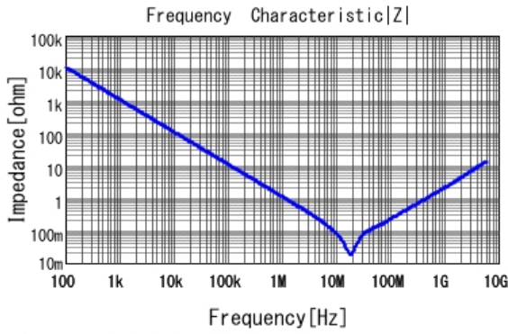
GCM188R71E154KA37 |Z| DCOV, 25degC
