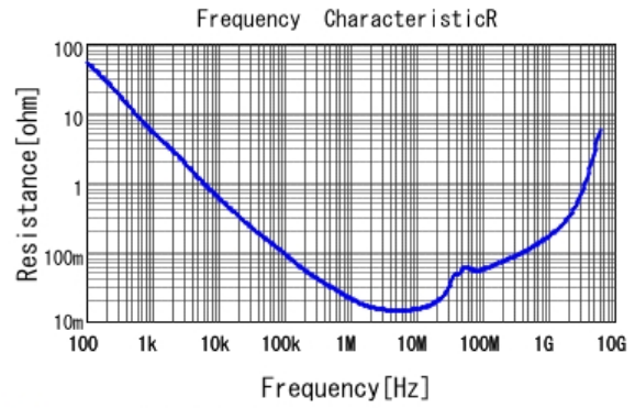
GCM188R71E154KA37 R DCOV, 25degC
