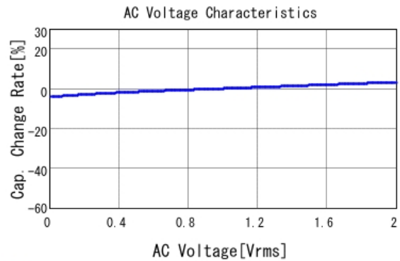
GCM188R71E154KA37 C-AC Voltage capchange, DCOV, 25.0d
