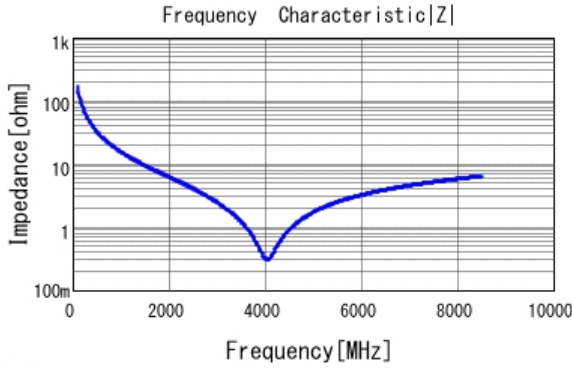
■ GRM0225C1H9R6WA03 |Z| DCOV, 25degC
