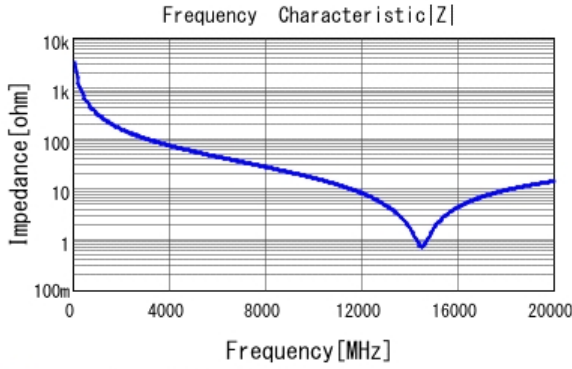
■ GRM0225C1HR50WA03 |Z| DCOV, 25degC
