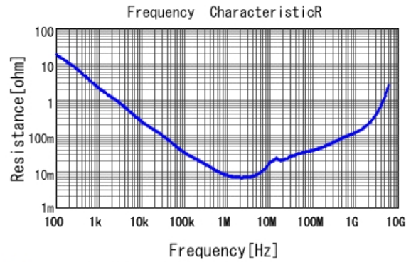
■ GRM188C81C225KA12 R DCOV, 25degC
