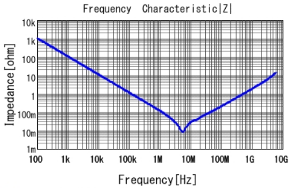
■ GRM188C81C225KA12 |Z| DCOV, 25degC
