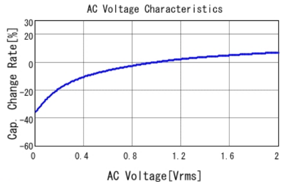
■ GRM188C81C225KA12 C-AC Voltage capchange, DCOV, 25.0d
