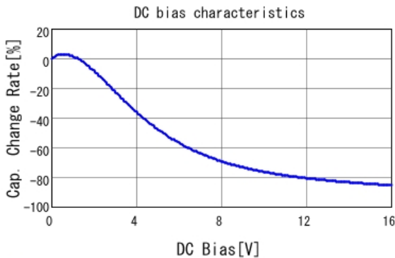
■ GRM188C81C225KA12 C-DC bias capchange, 25.0degC, AC1.
